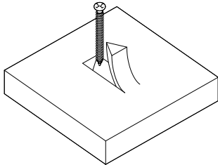
Glue-free and concealed mounting with patented Undercover system.
