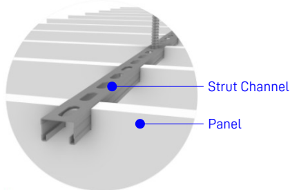
Baffle Mounting Detail:
