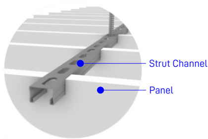
Baffle Mounting Detail:
