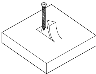
Glue-free and concealed mounting with patented Undercover system.
